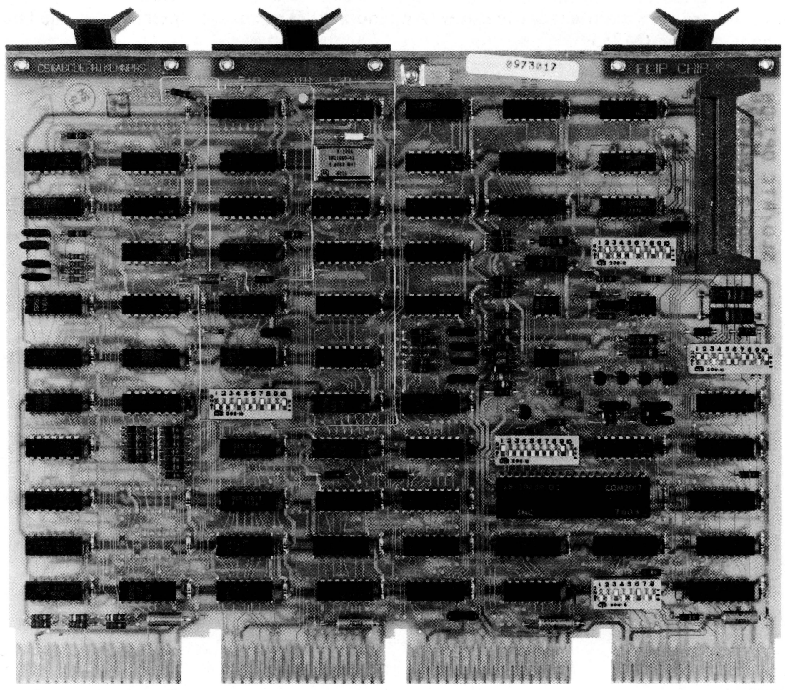
Figure 1-12 DL11-W Serial Line Interface and Real-Time Clock
