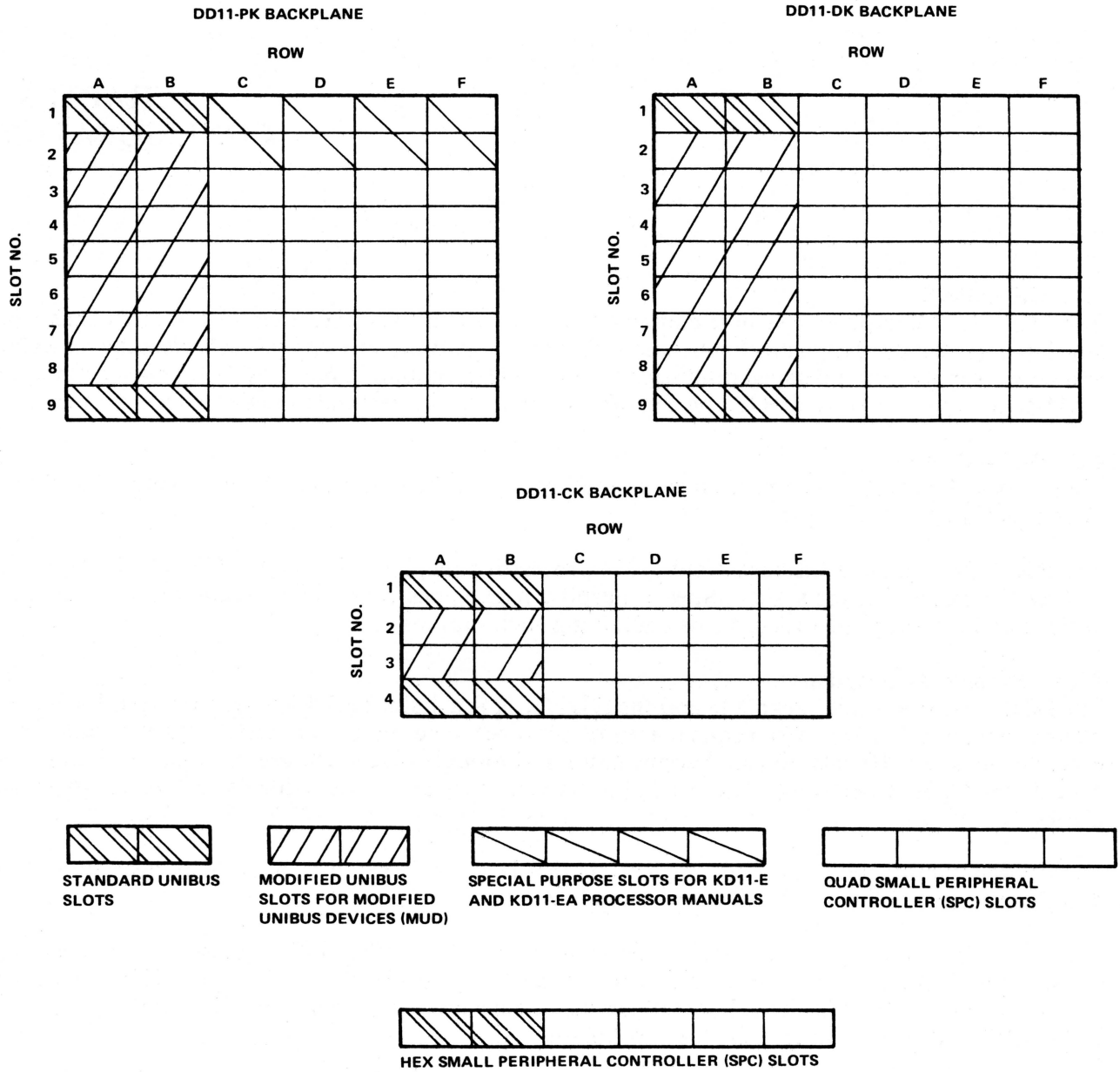
Figure 4-1 PDP-11/34 Backplanes
