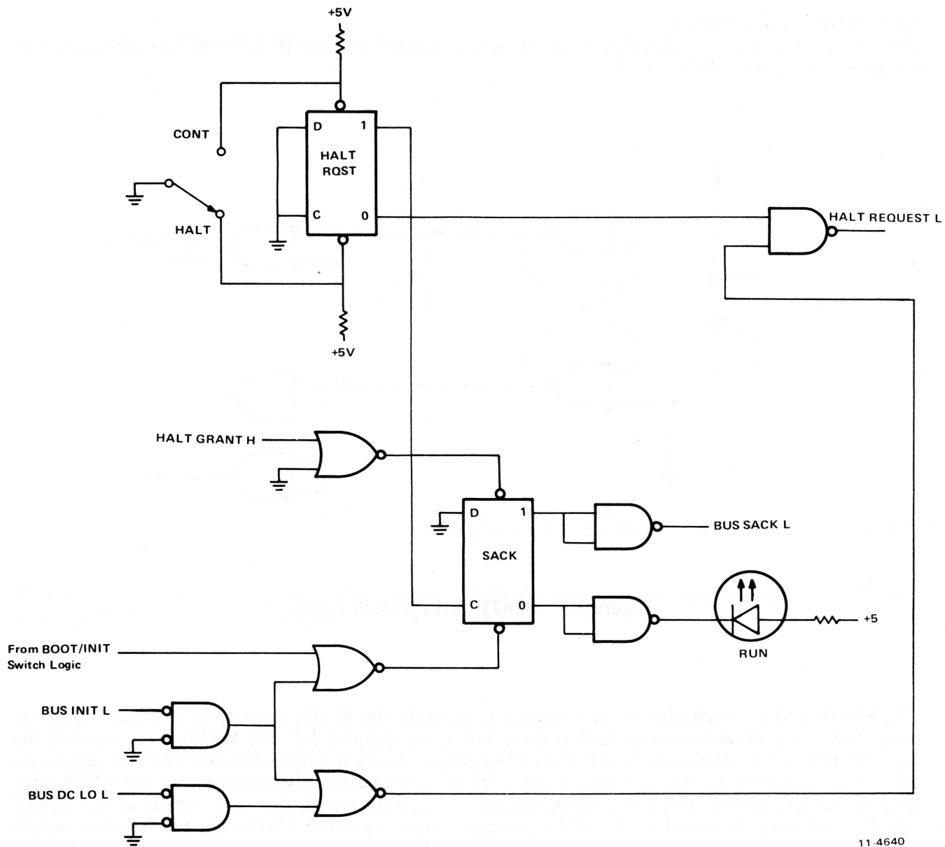
Figure 3-4 HALT/CONT Switch Logic
