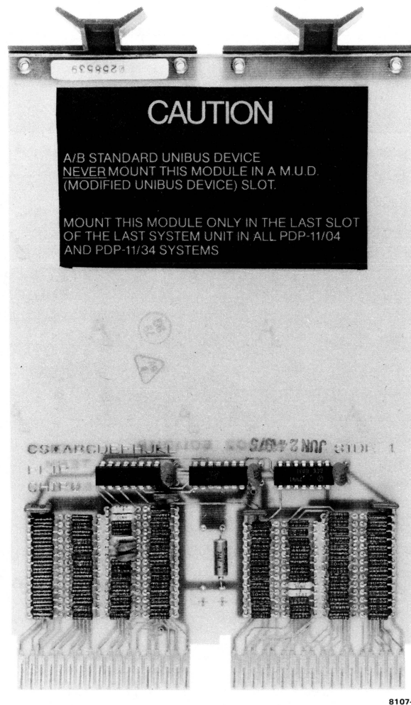
Figure 1-7 M9302 Terminator Module
