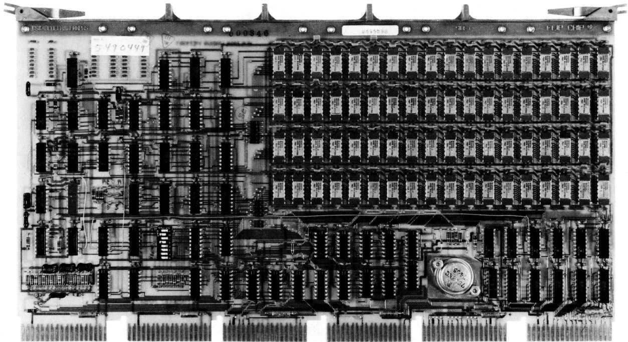
Figure 1-8 MS11-JP MOS Memory Module
