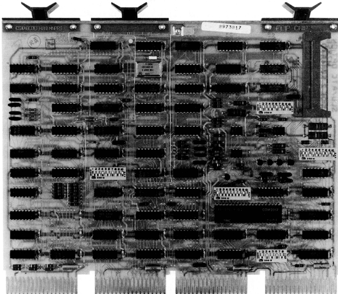
Figure 4-9 DL11-W (M7856) Switch Locations
