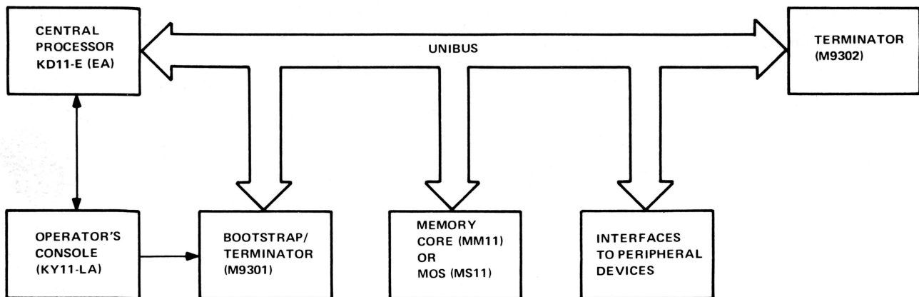
Figure 1-2 System Block Diagram
