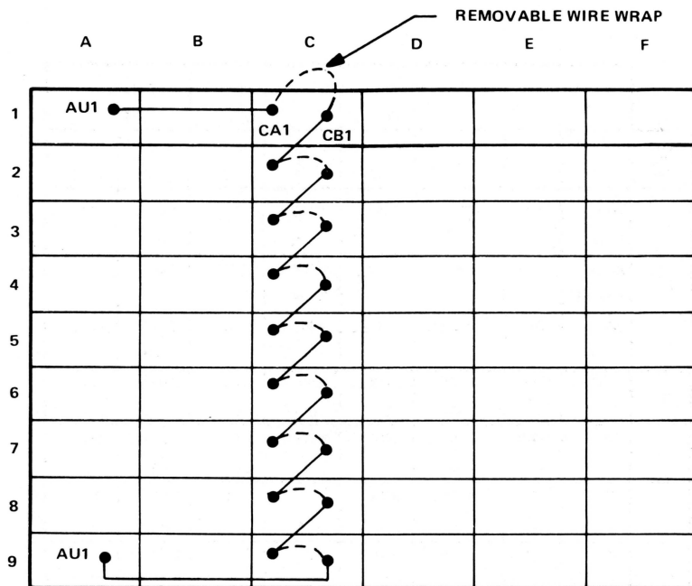
Figure 4-6 NPG Signal Path
