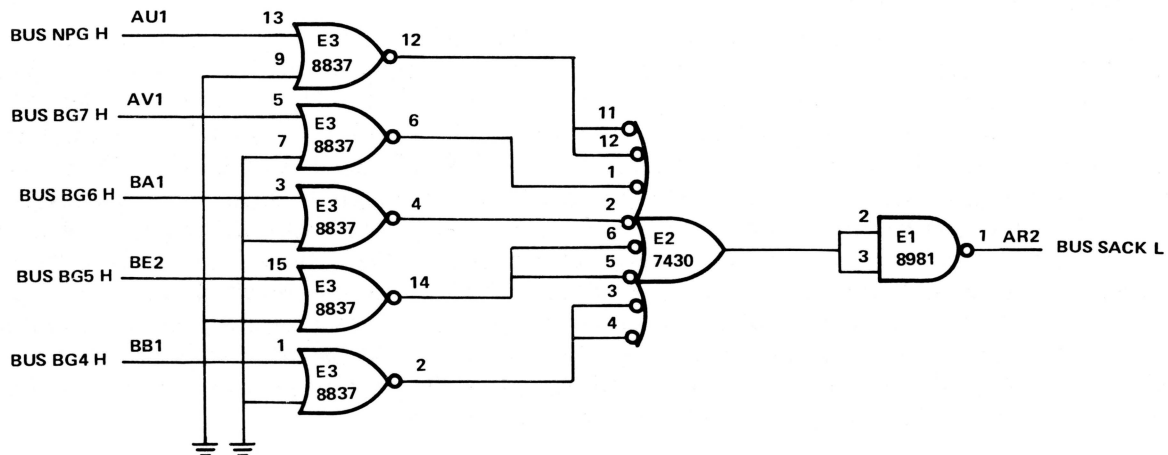
Figure 3-3 M9302 Sack Turnaround Logic
